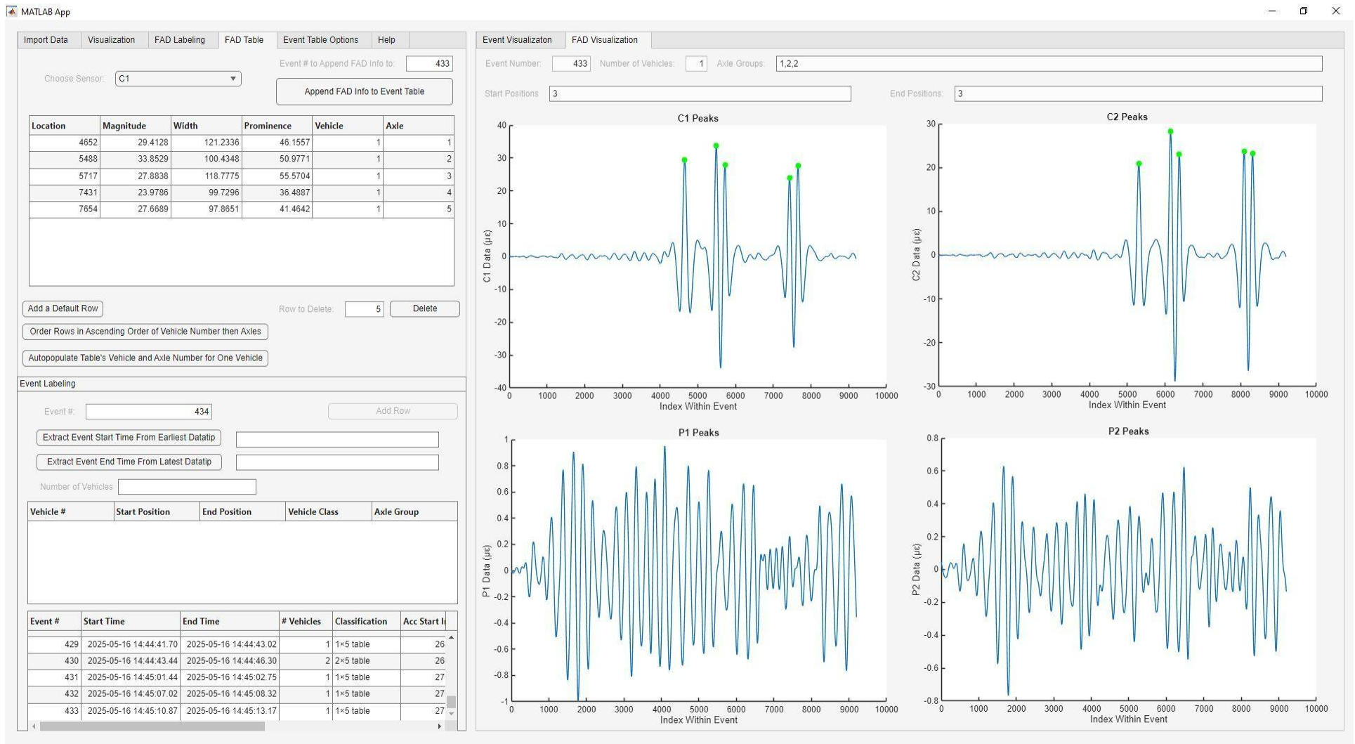
Figure 2: MATLAB App (2/2)
