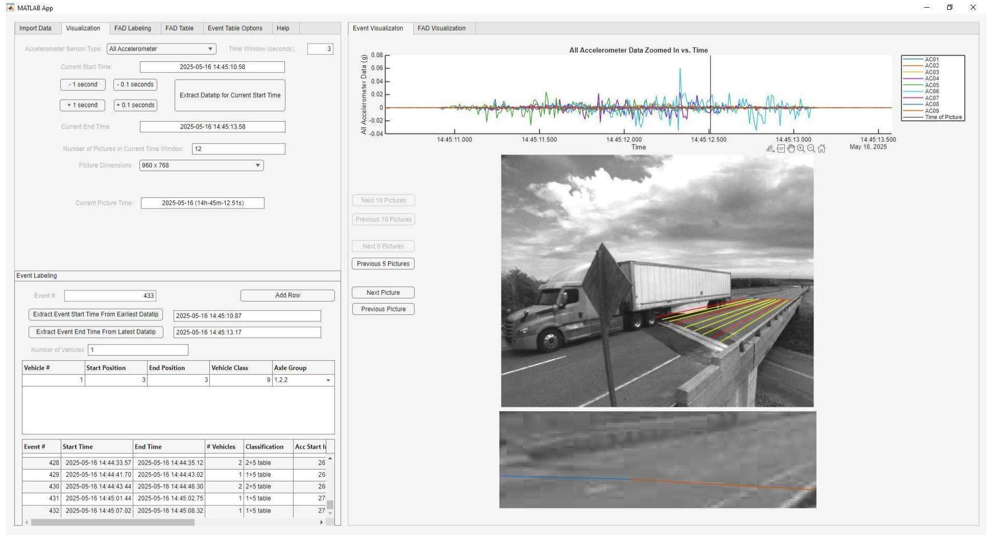
Figure 1: MATLAB App (1/2)
